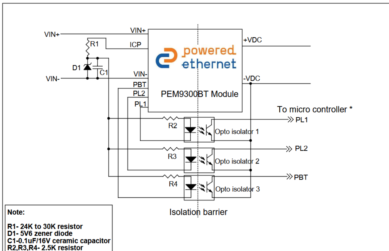
Figure 4- Power level indication connections to host-board
