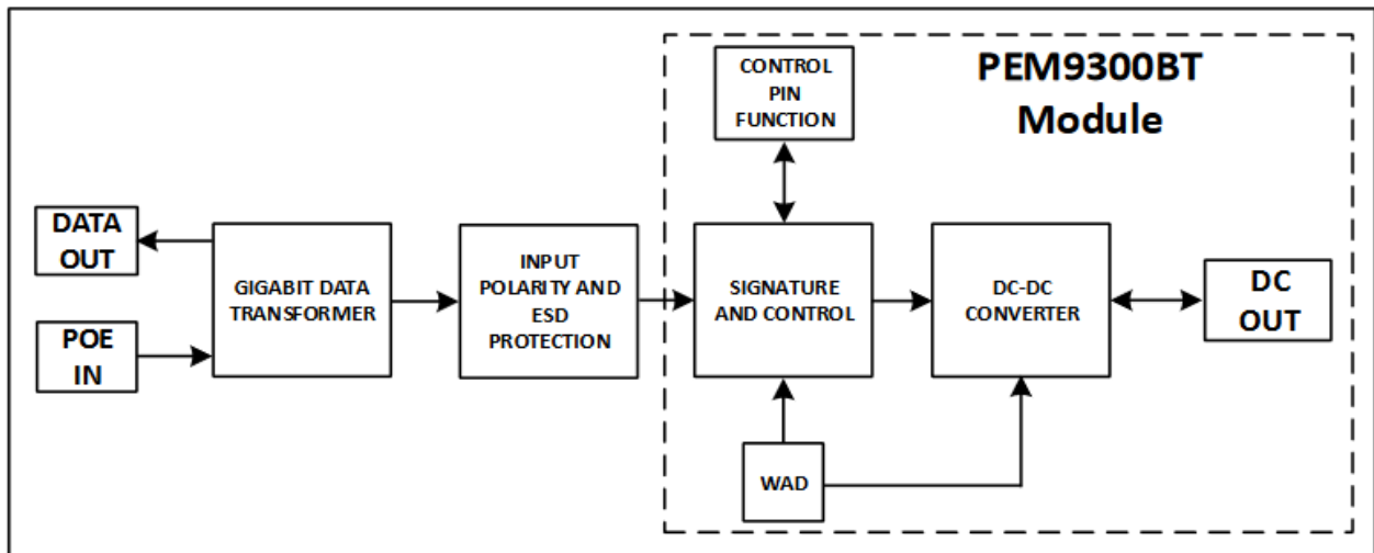
Figure 3- Block Diagram
