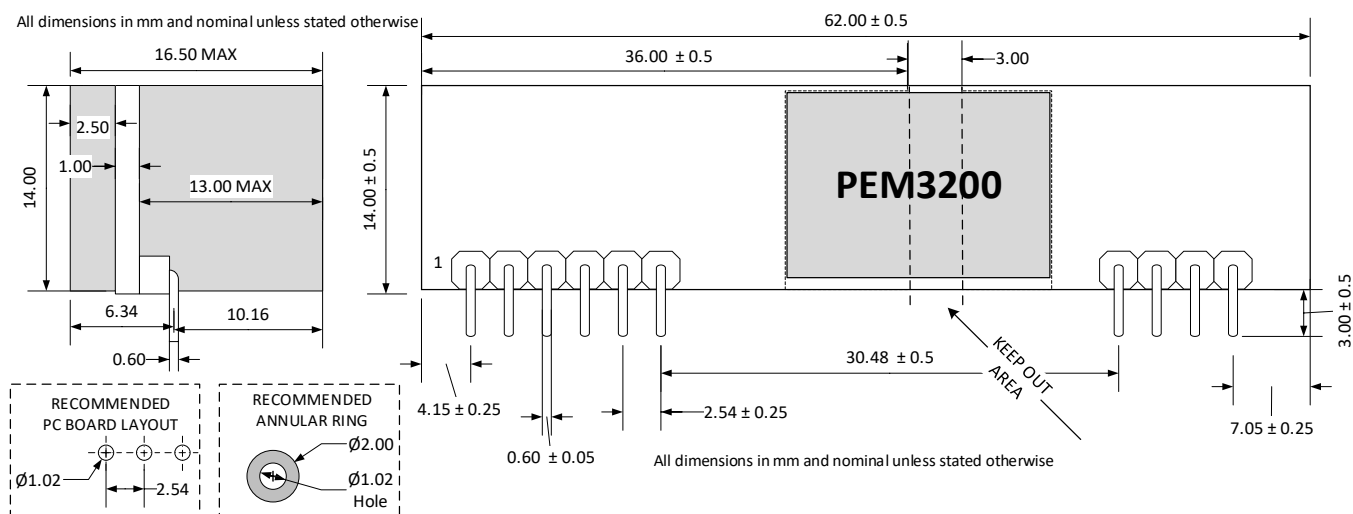
Figure 9- Mechanical Dimensions
