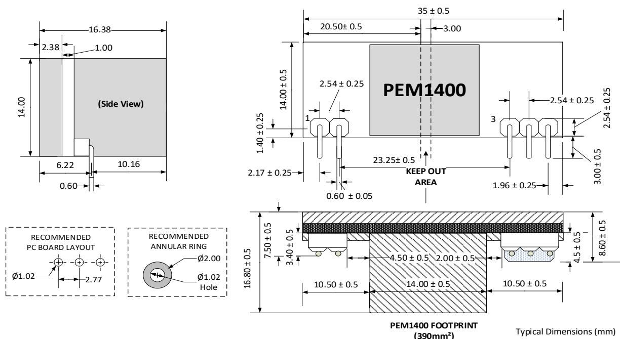
Figure 19- Mechanical Dimensions
