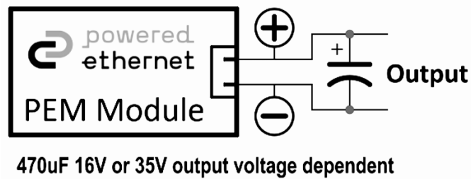
Figure 2- Output Connection
