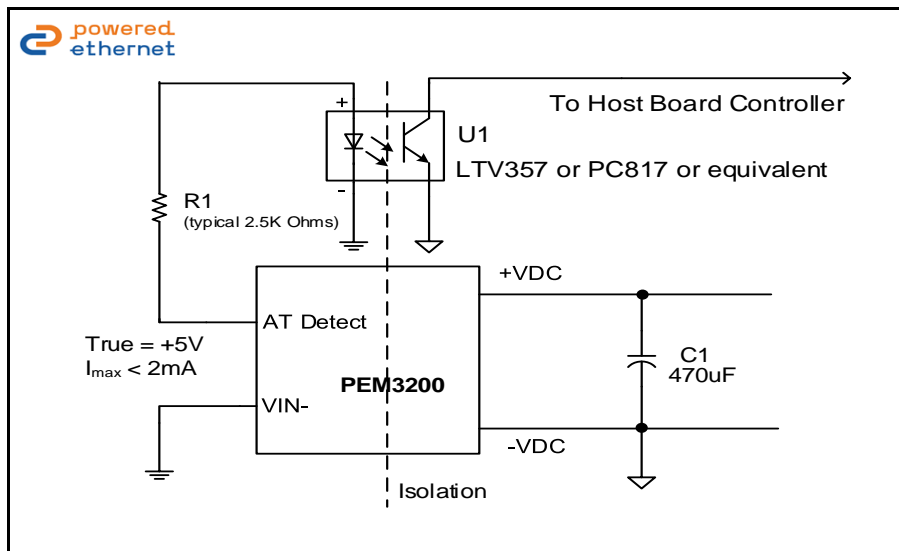
Figure 5- AT Detect Pin Connection
