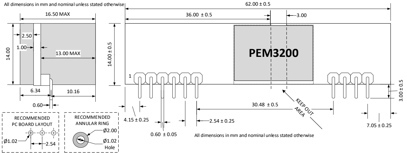
Figure 9- Mechanical Dimensions
