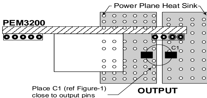
Figure 8- Power Plane Heat Sink
