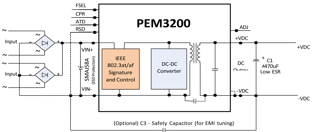
Figure 3- Block Diagram
