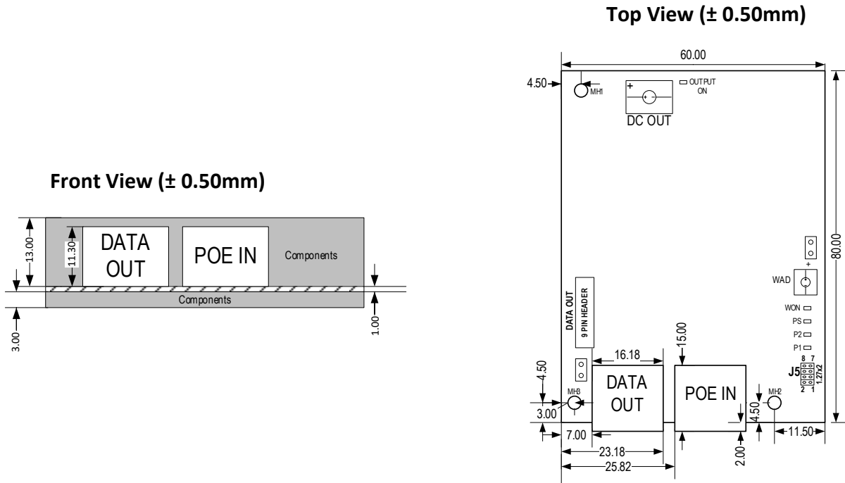
Figure 4- Mechanical Dimensions
