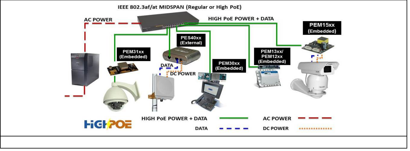
Figure 6 – Typical PoE System Configuration
